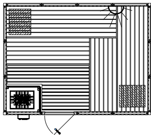
SA-20 / 275 x 210 x 206 / 7 Kw
