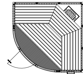
SA-18P / 215 x 215 x 206 / 6 Kw
