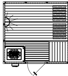
SA-17 / 210 x 194 x 206 / 6 Kw
