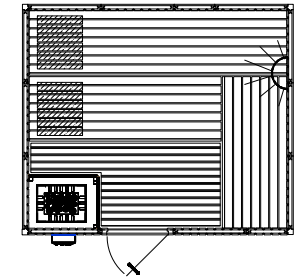
SA-19 / 245 x 210 x 206 / 7 Kw
