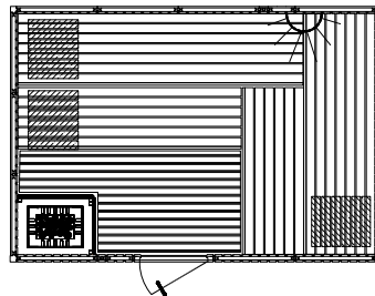
SA-21 / 303 x 210 x 206 / 8 Kw
