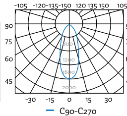
LC2X24W-BF 6400°
