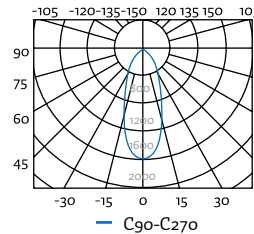
LC3X24W-BF 6400°
