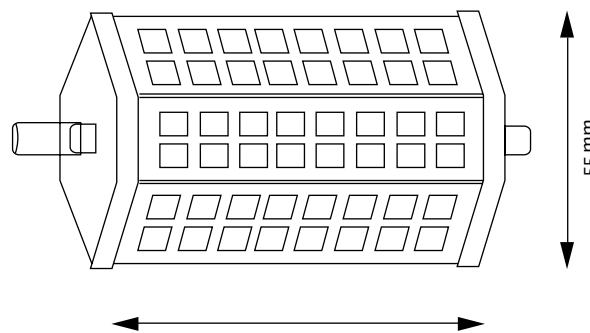
R7S-78BC=78mm R7S-118BC=118mm R7S-189BC=189mm
